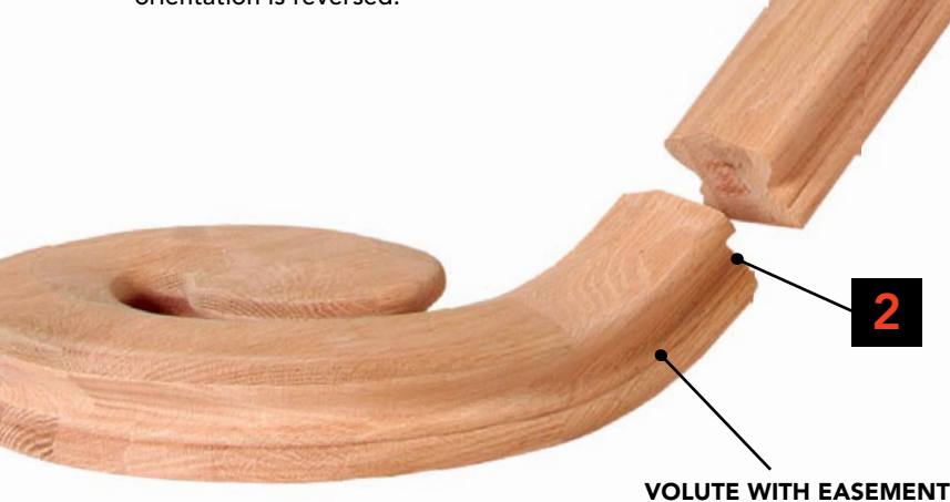
Removable pitch blocks
